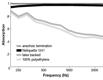
Acoustical Performance for Panel Applications (ISO 10534-2)
